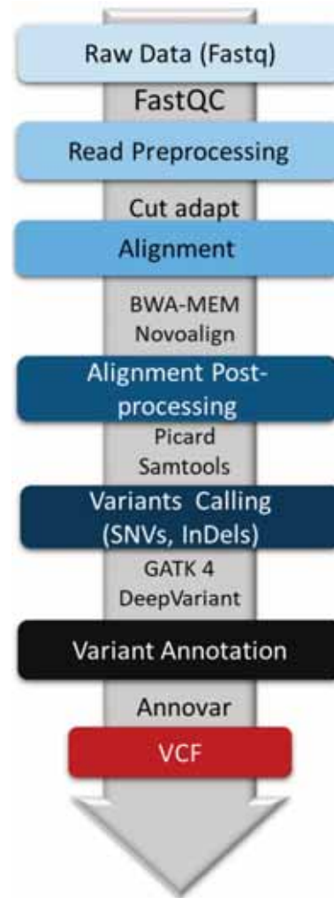
Figure 2. Exome/Genome Data Analysis Pipeline
