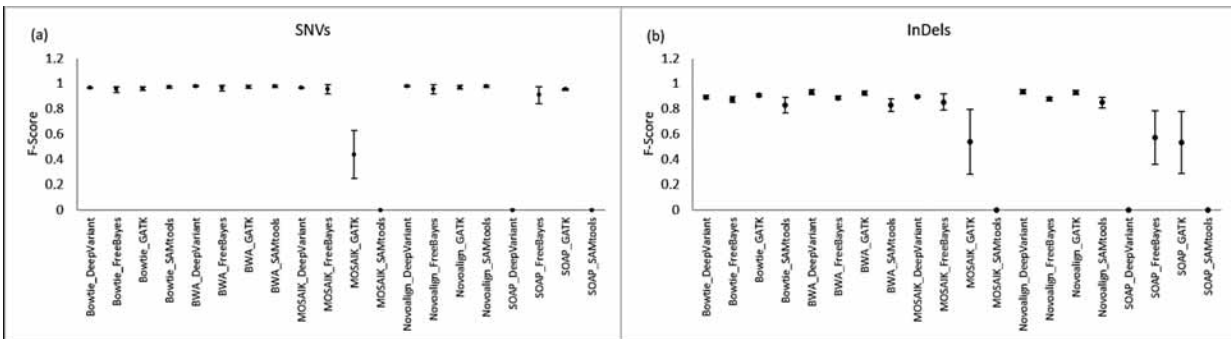
Figure1. Performance comparison of pipelines with respect to F-score on NA12878, NA24385, and NA24631. DeepVariant performed best invariably with all data sets. However, the aligners BWA and Novoalign both performed equally well on the new datasets compared with NA12878. The values and the error bars represent the average and standard deviation respectively of F-score obtained from all 3 datasets. Performance comparison of pipelines in SNVs and InDels detection for GRCh38 (a, b).
